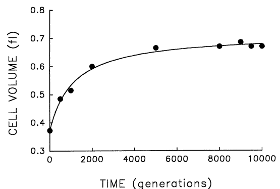
FIG. 1. Trajectory for average cell volume in one population of E. coli during 10,000 generations of experimental evolution. Each point is the mean of two assays. Curve is the best fit of a hyperbolic model. Averages were calculated after removing particles of <0.25 fl, except for the ancestor ( t = 0 ) where particles of <0.15 fl were removed; these criteria gave a clear separation between cells and background particles. Cell sizes were measured in stationary-phase populations, at the end of the 24-h serial transfer cycle.
